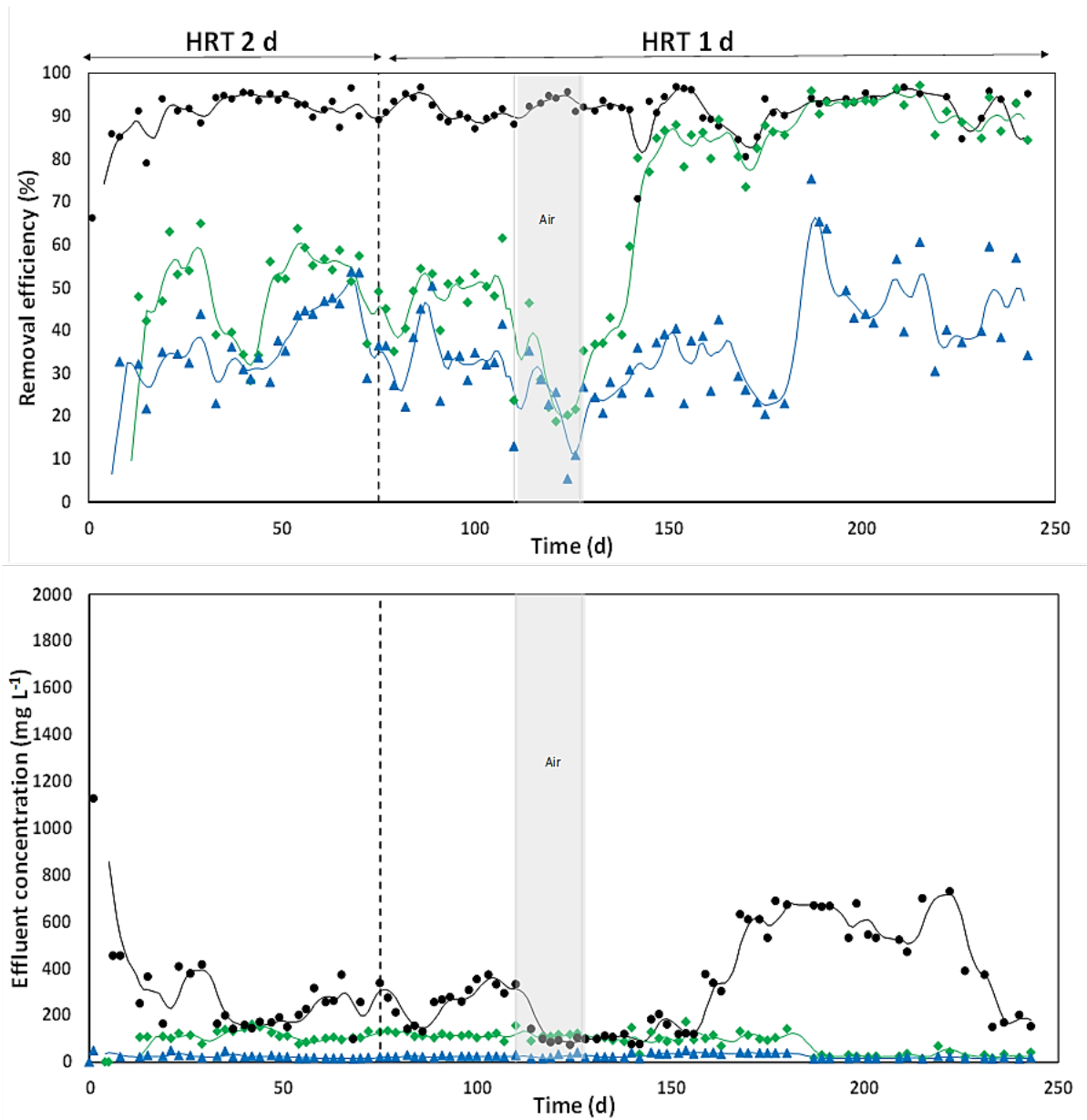
Figure 15. Performance for treatment to remove TCOD (●), TN (◆) and TP (▲), showing removal efficiencies (top) and effluent concentrations (bottom) with PPB as the biomass being grown (solid lines represent a 5 d moving average).
