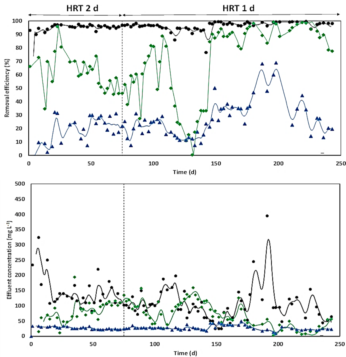
Figure 16. Performance for treatment to remove TCOD (●), TN (◆) and TP (▲), showing removal efficiencies (top) and effluent concentrations (bottom) with microalgae as the biomass being grown (solid lines represent 5 d moving average).
