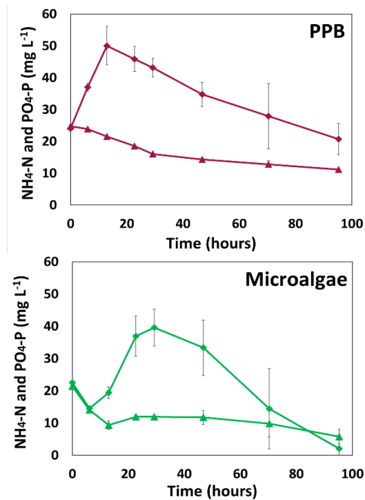
Figure 12. Time trend measurements of \text{NH}_4\text{-N} ( \blacklozenge ) and \text{PO}_4\text{-P} ( \blacktriangle ) for treatment of poultry processing wastewater by growing (top, red) PPB or (bottom, green) microalgae. Additional data are provided in Hülsen et al. (2018a).
