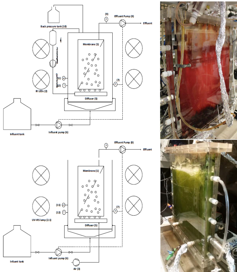
Figure 2. Schematics and photos of the laboratory-scale continuous wastewater treatment systems; (Top) PAnMBR growing PPB; (Bottom) PAMBR with microalgae and heterotrophs.
