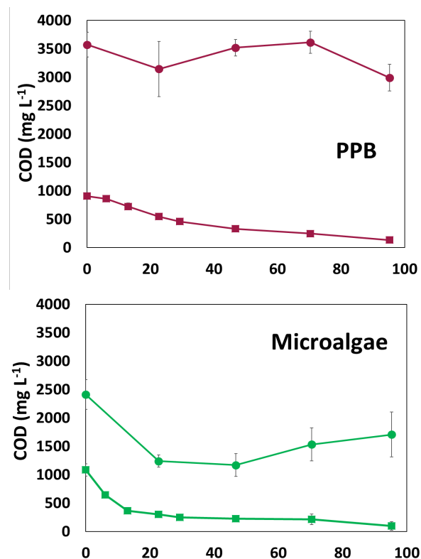
Figure 11. Time trend measurements of tCOD (●) and sCOD (■) for treatment of poultry processing wastewater by growing (top, red) PPB or (bottom, green) microalgae. Additional data are provided in Hülßen et al. (2018a).
